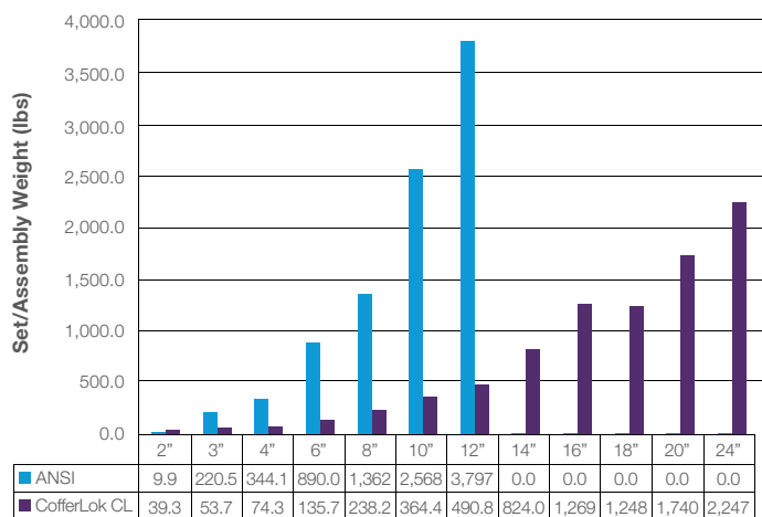
2500# Class Comparison
