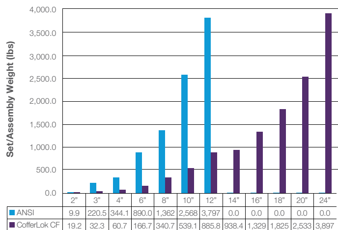
2500# Class Comparison
