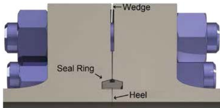
BEFORE ASSEMBLY
