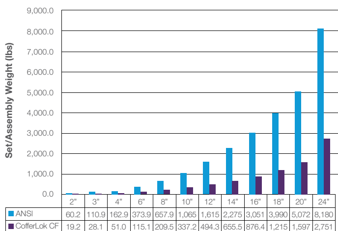
1500# Class Comparison
