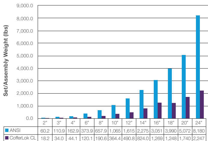
1500# Class Comparison
